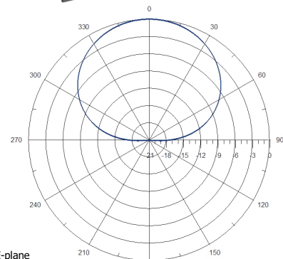
E-plane Horizontal Pattern
